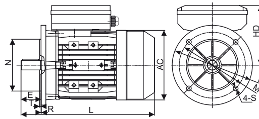
FLANGE MOUNTED B5
