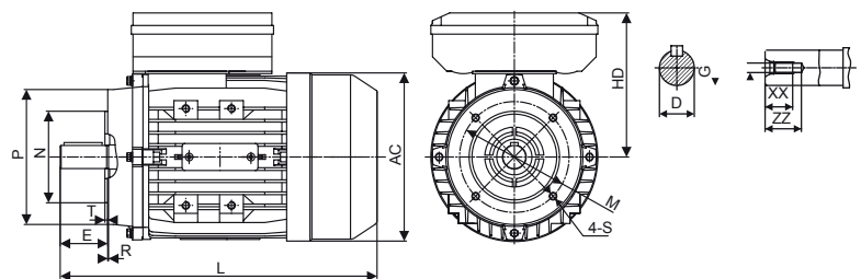
FOOT & FLANGE MOUNTED B14
