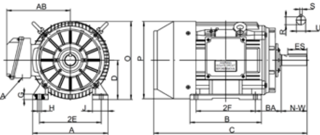
FOOT MOUNTED
